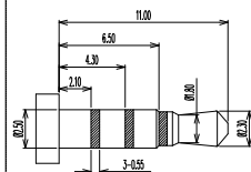
Ø2.50mm 4 POLE PLUG DETAIL
