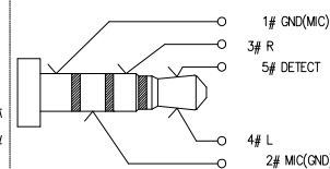
Ø2.50mm 4 POLE PLUG SCHEMATIC
