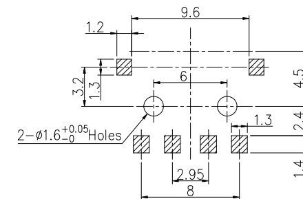
P.C.B.MOUNTING DETAIL
